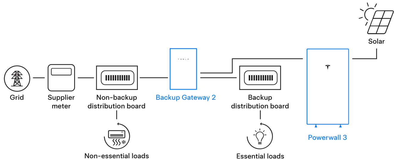
Figure 3. Partial Home Backup with Loads Upstream of Backup Gateway 2
